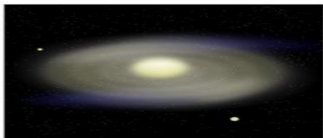
Physics scope ranges from macroscopic quantities like the universe and microscopic quantities like an atom
