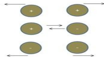
The unlike charges attract each other while like charges repel each other. A current carrying wire generates magnetic field around it, giving rise to electromagnetism.
