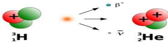
B-decay of a nucleus.
